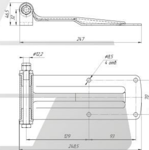
F05 Hinge (Zn, SS) – 6306034-12
