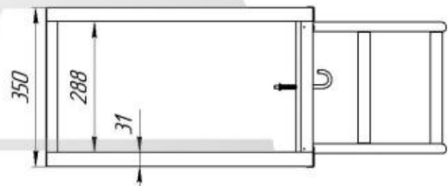
A84 Sliding 2 step rear ladder H=588 AC 02.00.000
