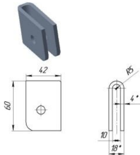
Lever mount 6306038.002
