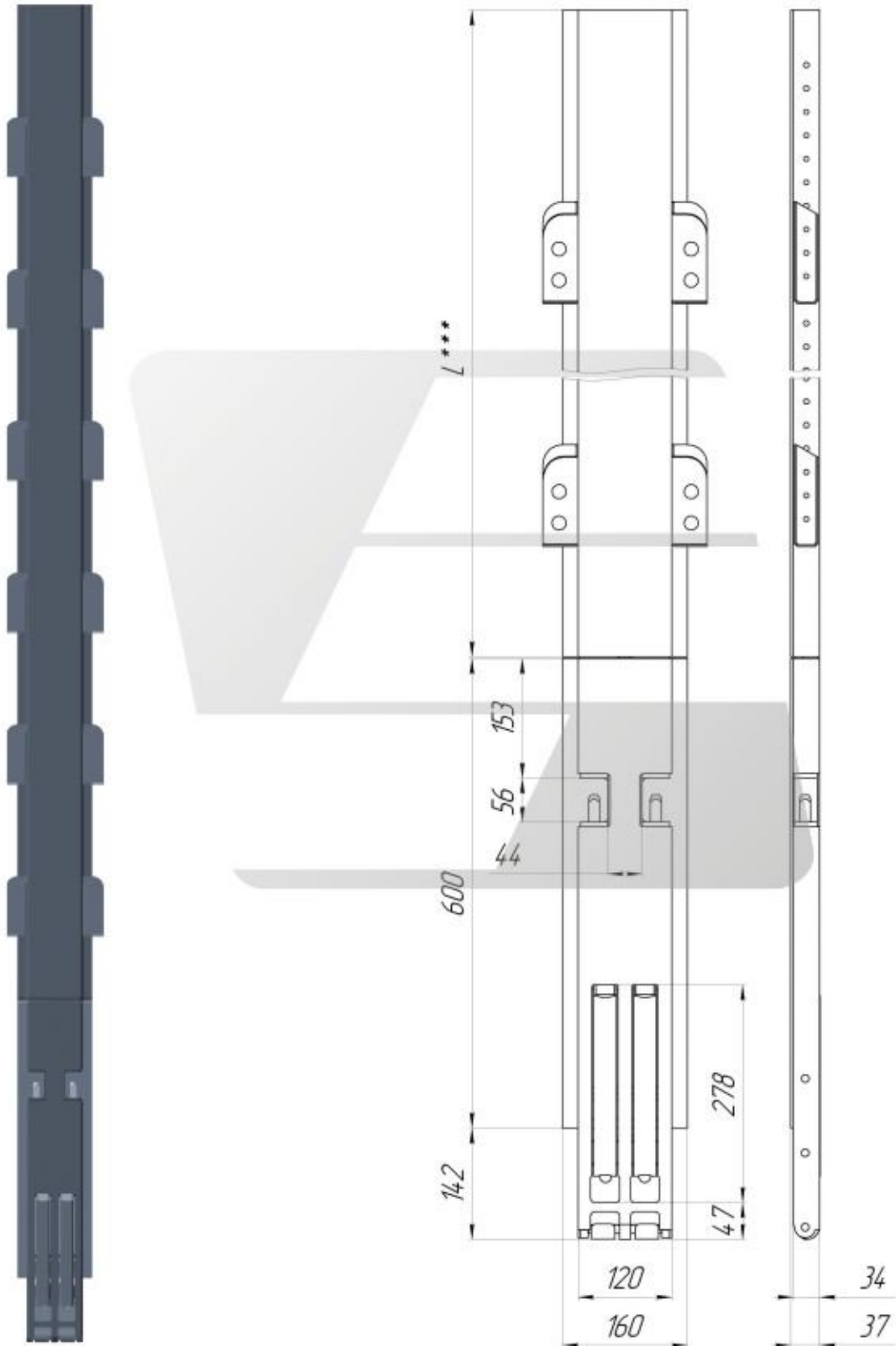
P113 Folding curtainside pillar series 600 with elongated channel and pockets
