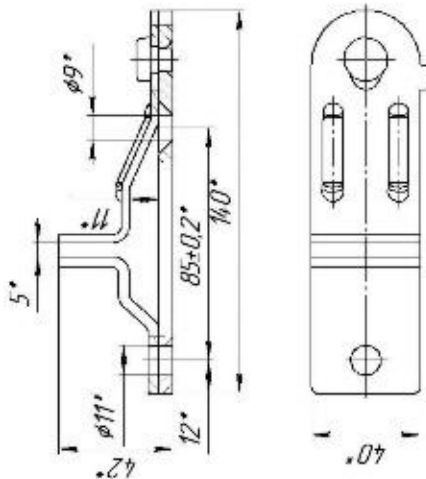
Lever retainer 6306037
