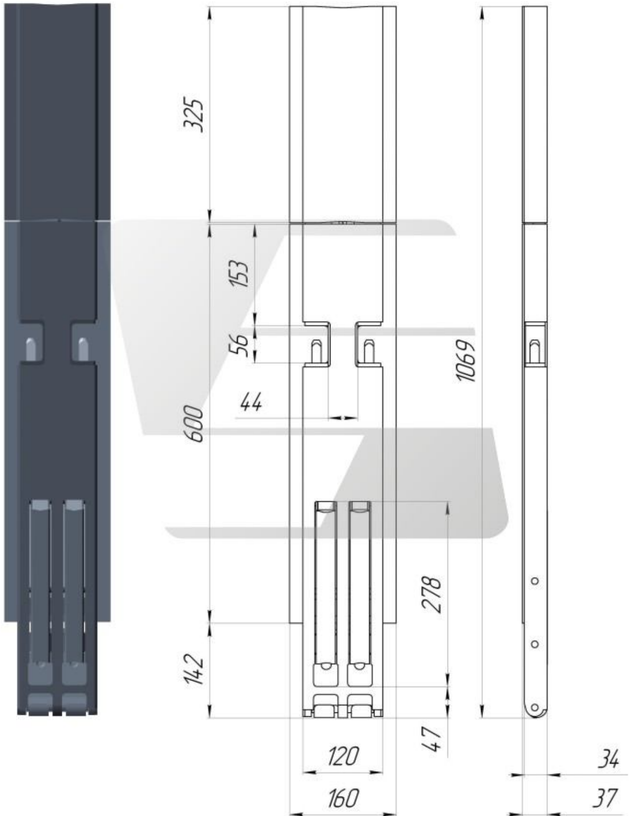
P112 Folding curtainside pillar series 600
