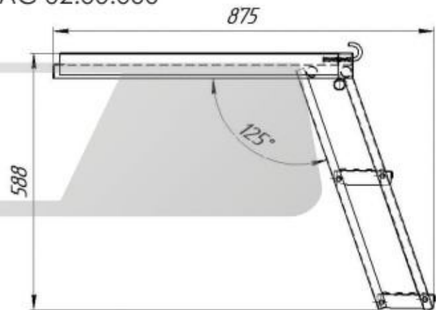
A84 Sliding 2 step rear ladder H=588 AC 02.00.000
