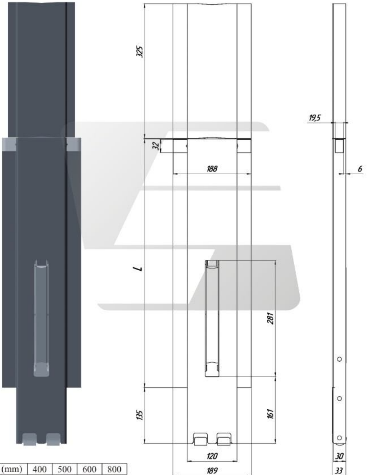
P124 Intermediate curtainside pillar for aluminum boards 120 mm width
