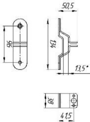
Lever retainer 6305416-03
