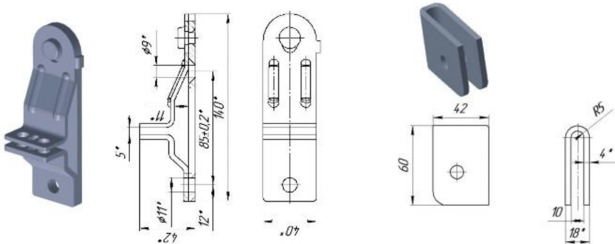
Lever retainer 6306037
