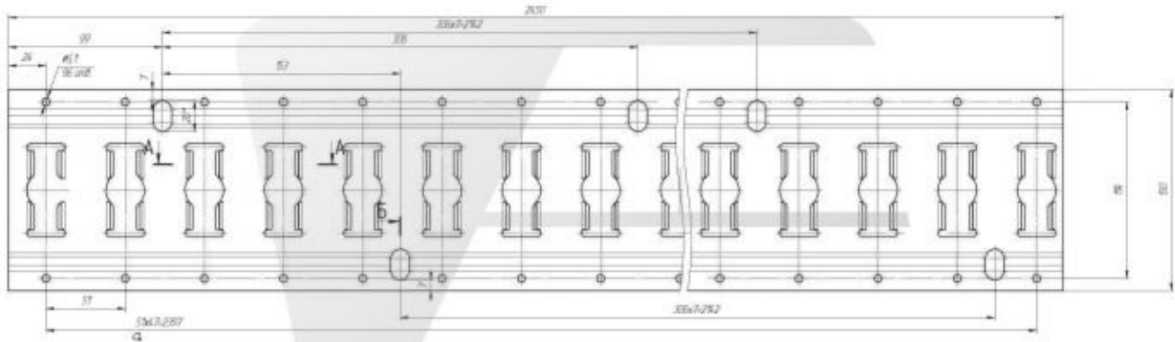
L92 Recessed swing
