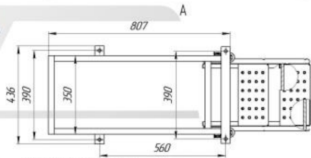
A82 Rear ladder with narrow steps AC 03.00.000
