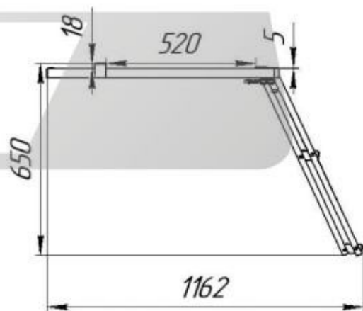
A82 Rear ladder with narrow steps AC 03.00.000
