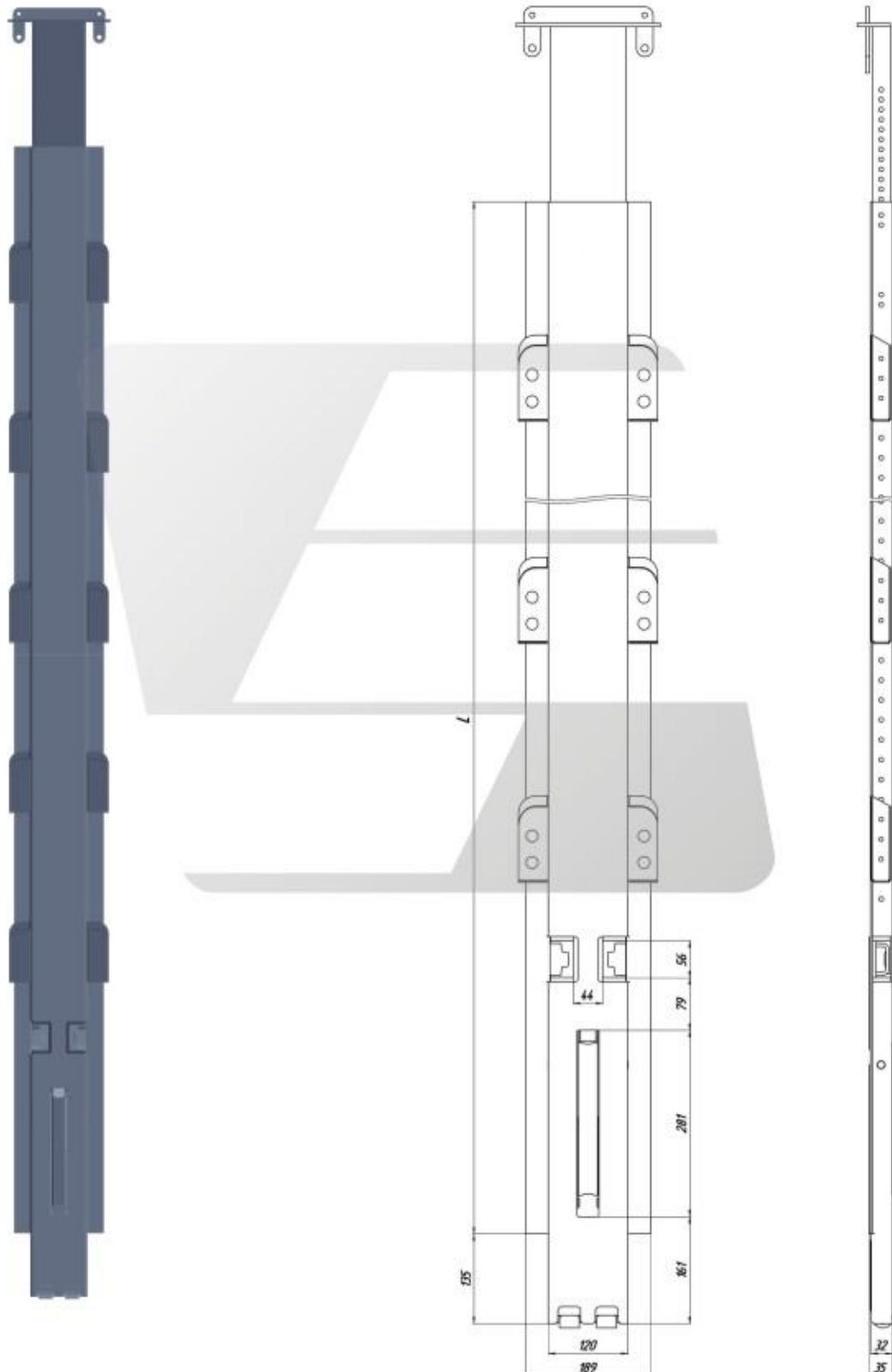
P132 Intermediate curtainside pillar for semitrailer with pockets and additional slots for swivel
