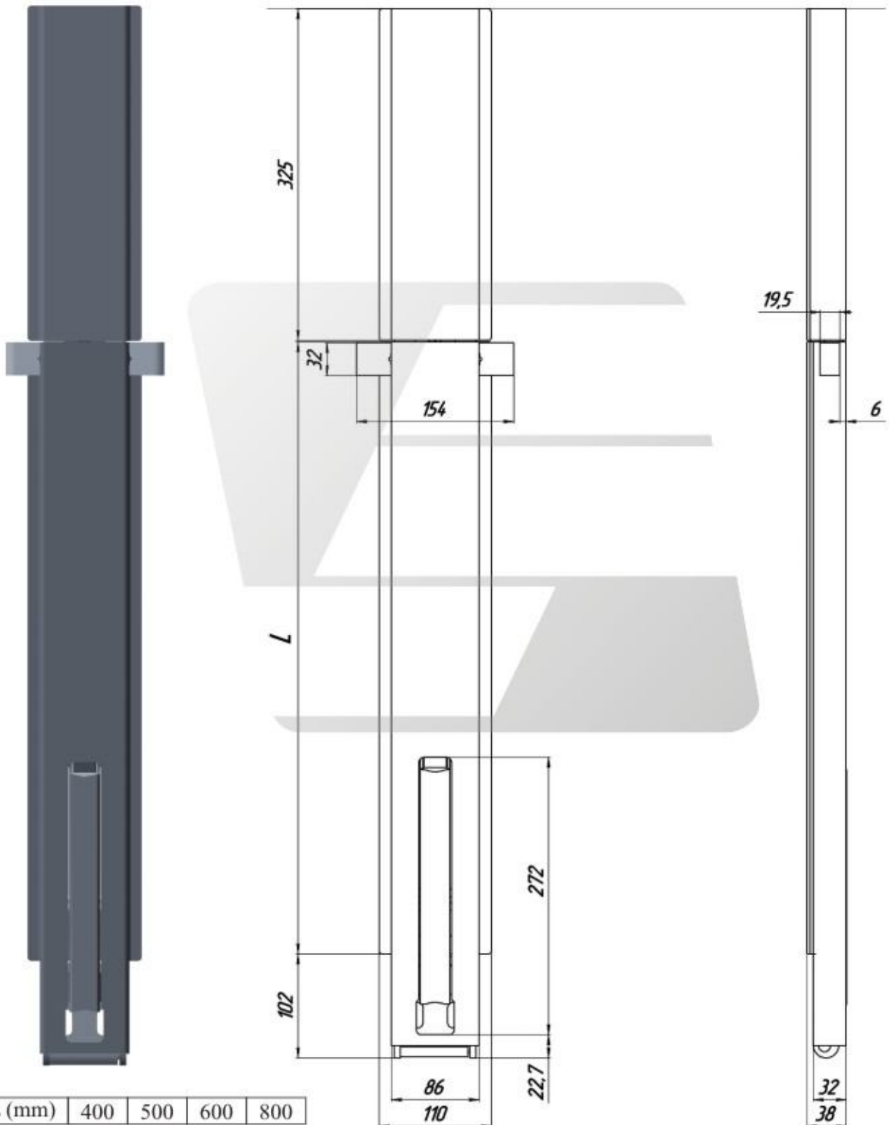
P123 Intermediate curtainside pillar for aluminum boards 86 mm width
