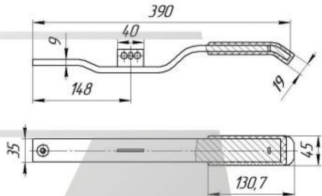
Lever mount 6306038.002
